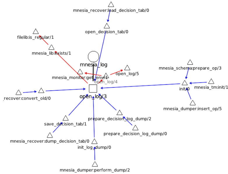
Figure 13: open_log/3 function call graph
