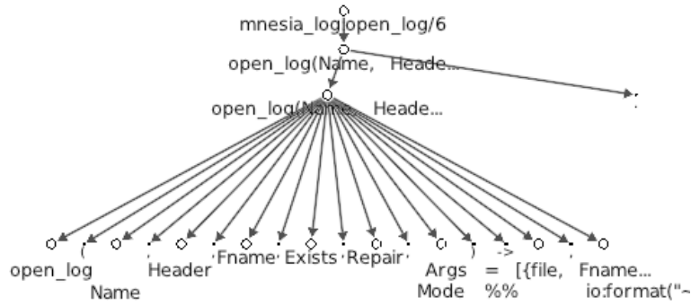
Figure 16: open_log/6 high level syntax view
