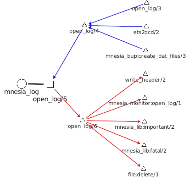
Figure 15: open_log/5 function call graph (layered view)
