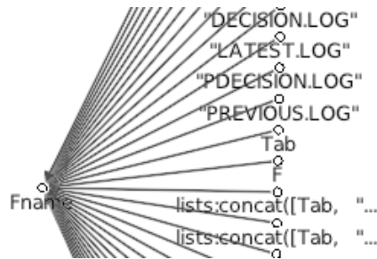
Figure 21: Exploring the values of the variable Fname
