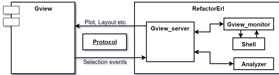
Figure 10: Our graph visualisation architecture, Gview.
