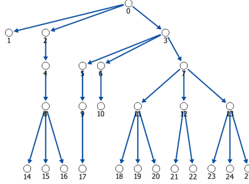
Figure 7: Layered layout
