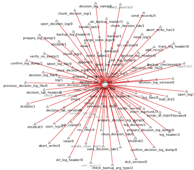
Figure 12: mnesia_log view
