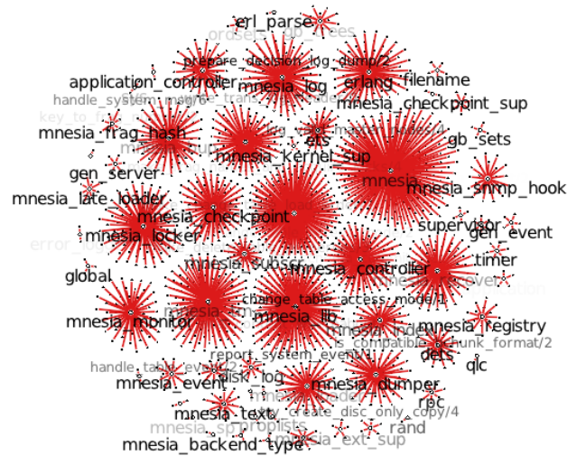
Figure 11: Mnesia view
