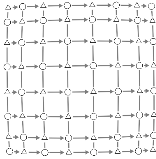
Figure 6: Force-directed layout
